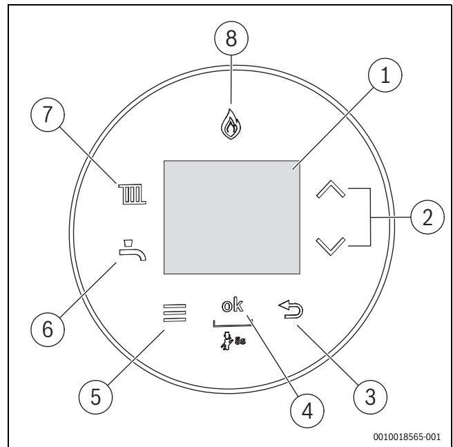
Fig. 7 Control panel
