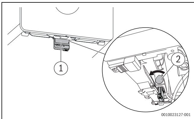
Fig. 9 Locking mechanism
