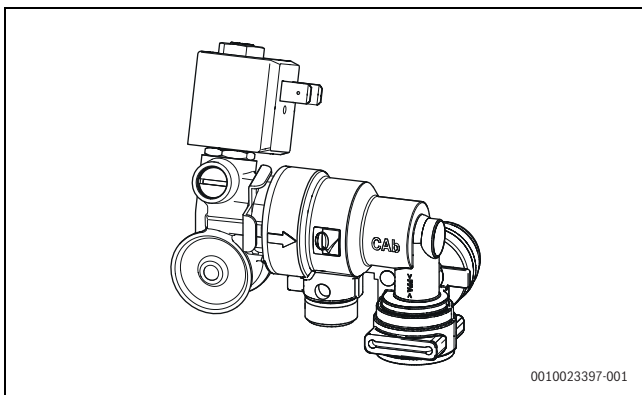
Fig. 6 Greenstar Intelligent Filling System
