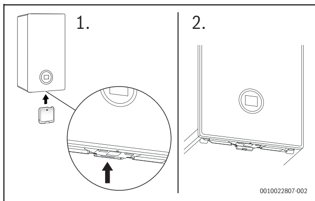
Fig. 8 Position of Key housing
