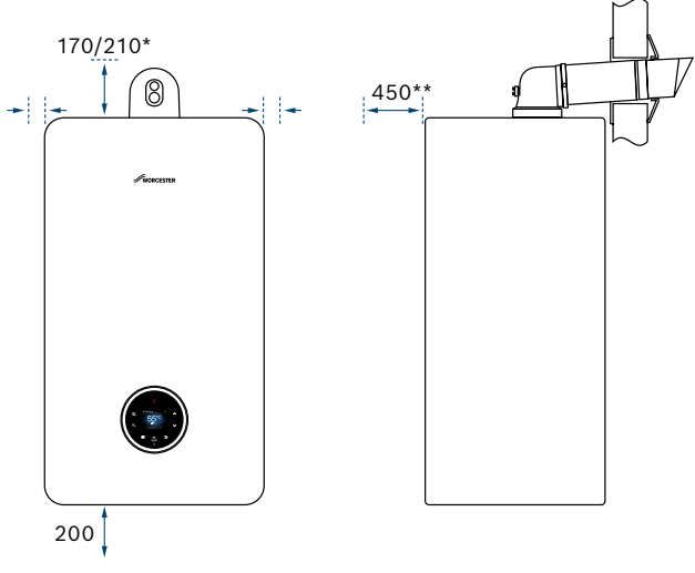
Clearances (mm)
